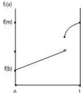
(c) The right-side function: f_2(x)
