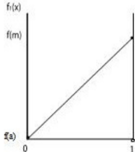
(b) The left-side function: f_1(x)
