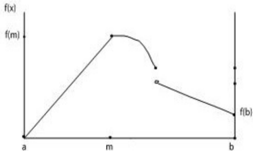
(a) The original f(x)
